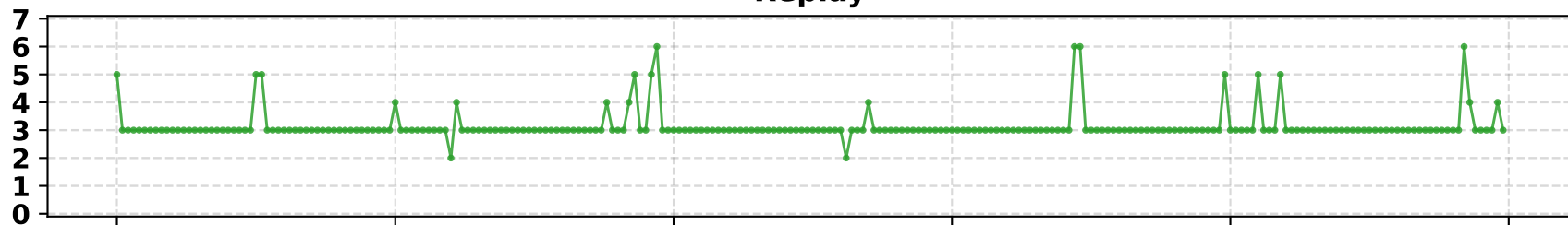
Replay
